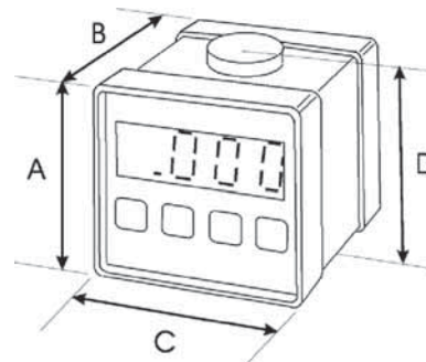
Loadblocks 2 and 5 tonne capacity
